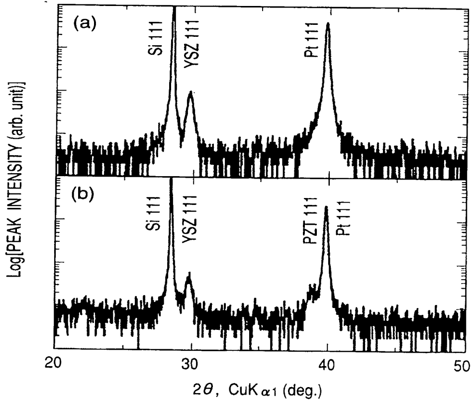
(a) (111)Pt//(111)YSZ//(111)Si SUBSTRATE (b) (111)PZT//(111)Pt//(111)YSZ//(111)Si SUBSTRATE
